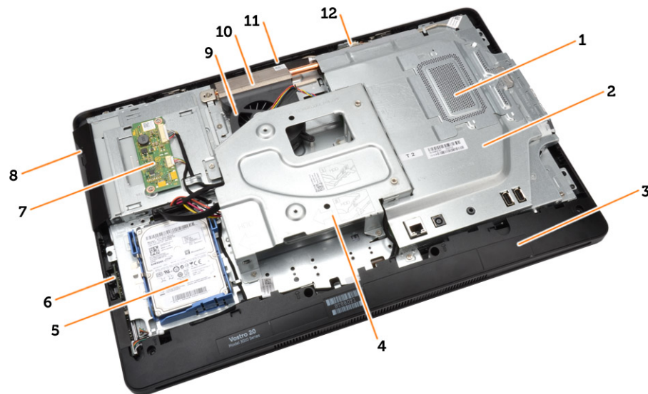
Figure 2. Inside View – 1
